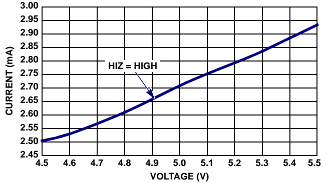
FIGURE 10. DISABLED SUPPLY CURRENT vs SUPPLY VOLTAGE
